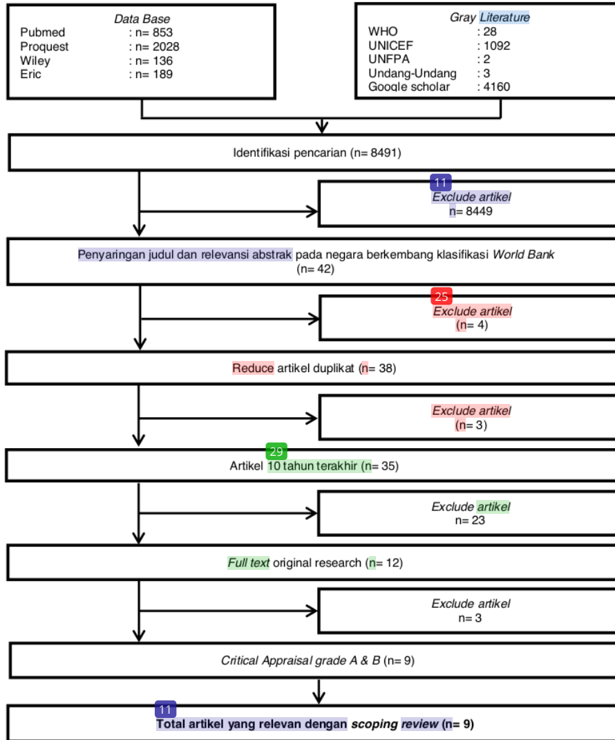
Gambar 1. Diagram PRISMA
