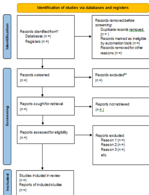
Gambar 1. Diagram PRISMA
